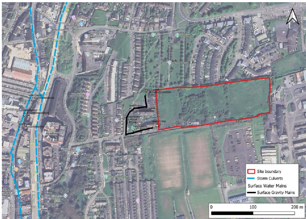
Figure 2-1: Existing storm drainage adjacent to site (extract from UE records, site boundary outlined in red)
