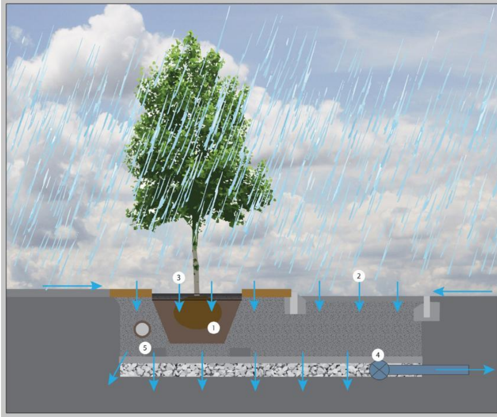
Figure 3-7 Tree Pit Schematic - Cross Section (ref: DMURS Advice Note 5)
