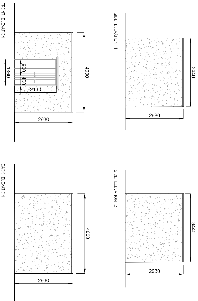
1no. Bin store to serve Block K
